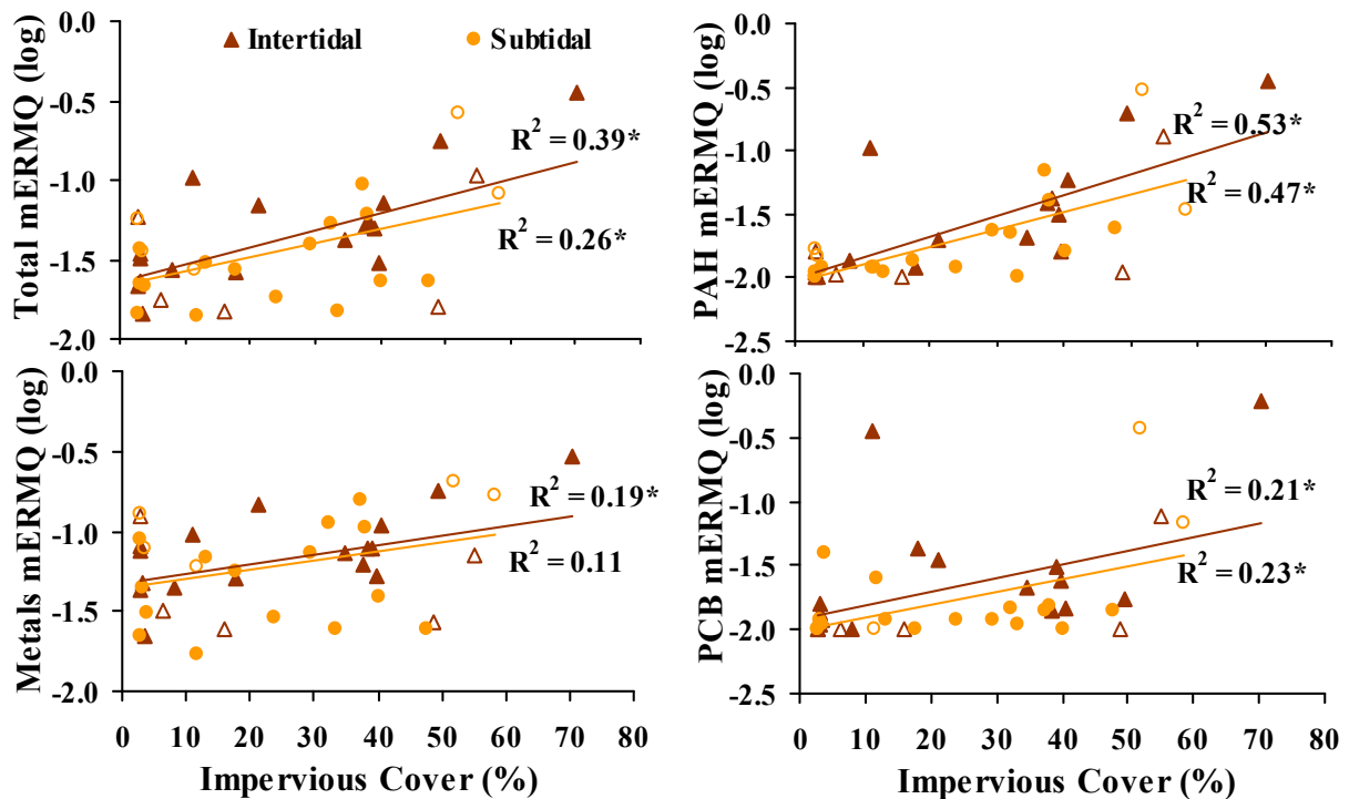
Figure 3-13. Relationship between mERMQ (log+0.01) and impervious cover for the study watersheds. Model R^2 is show for each regression with asterisk (*) indicating significance ( p < 0.05 ). Open markers represent GoM sites.
