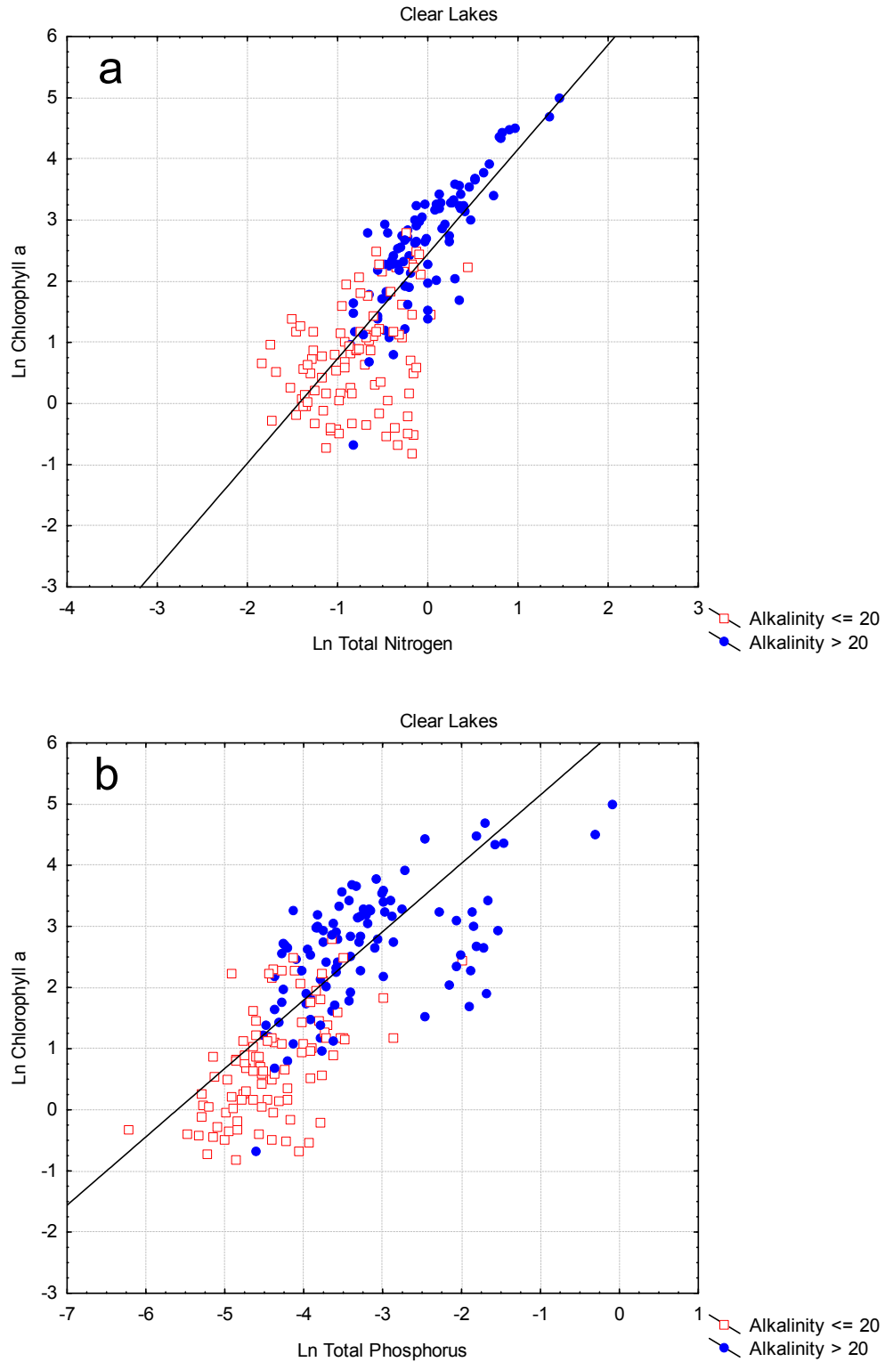
Figure 1-17. Scatter plot of annual geometric mean chl. a concentration and nutrients of clear lakes, showing separation of acidic and alkaline lakes with classification breakpoint at 20 mg/L CaCO 3 . Compare to Figure 1-5. Acidic and alkaline groups were combined in a single regression. a: TN; b: TP.
