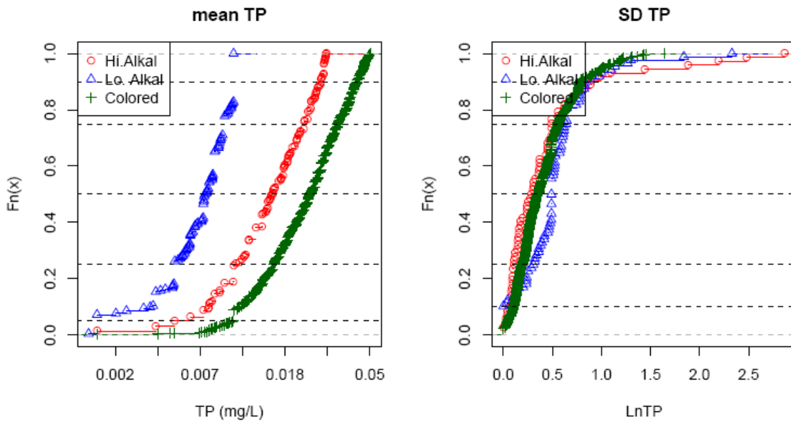
Figure 1-19. Cumulative frequency distribution of mean TP concentrations in acidic and alkaline lakes that meet the annual average criteria. A specific conductance > or < 250 \mu\text{S}/\text{cm} is applied as a threshold for classifying high- or acidic lakes.
