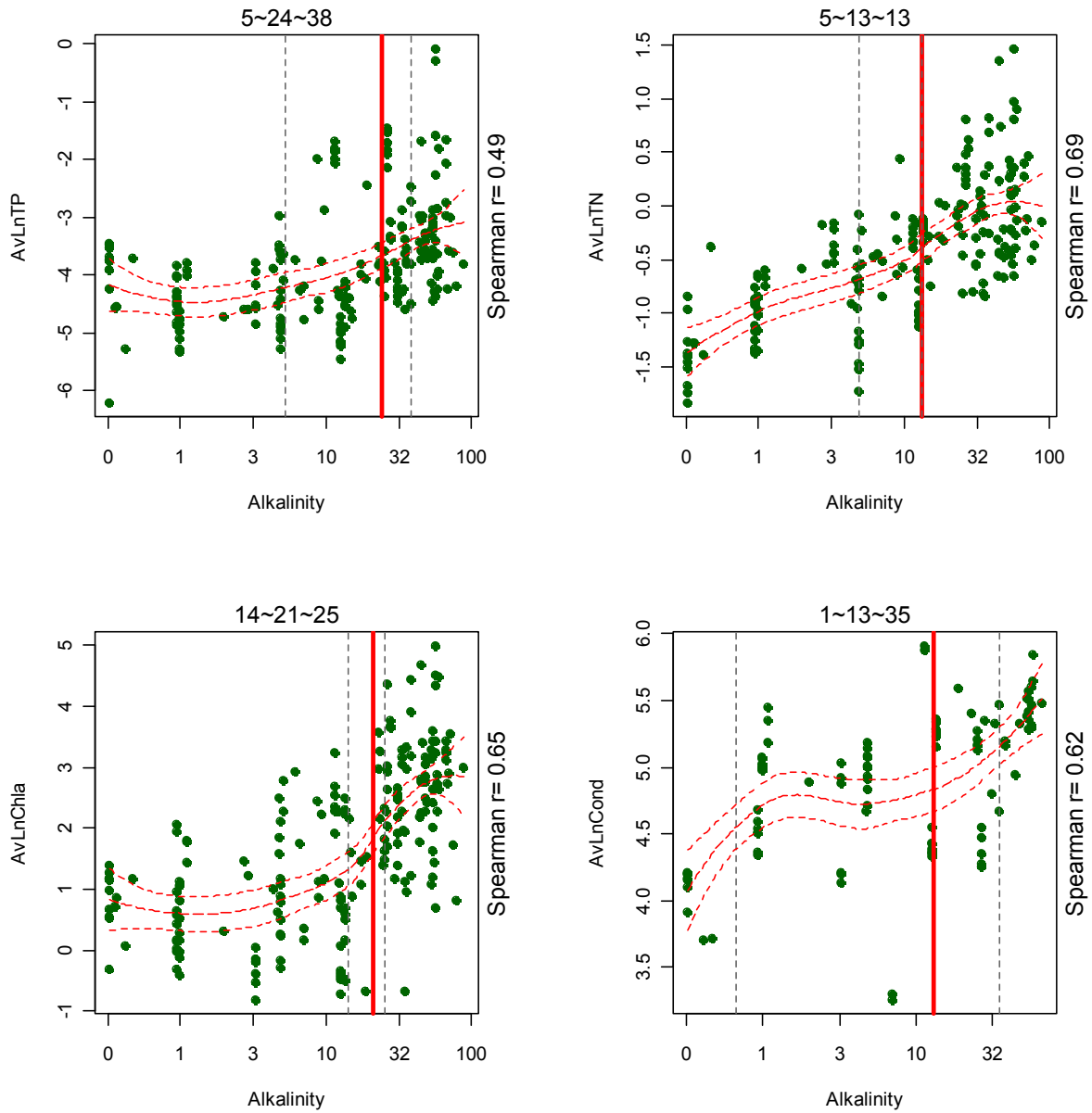
Figure 1-16. Scatterplots of mean TP, TN, Chl. a , and specific conductance on lake alkalinity. Vertical solid lines are the estimated change points, and vertical dashed lines denote the 95% confidence intervals for the change points. Wavy dashed lines are LOESS nonlinear regressions and confidence intervals.
