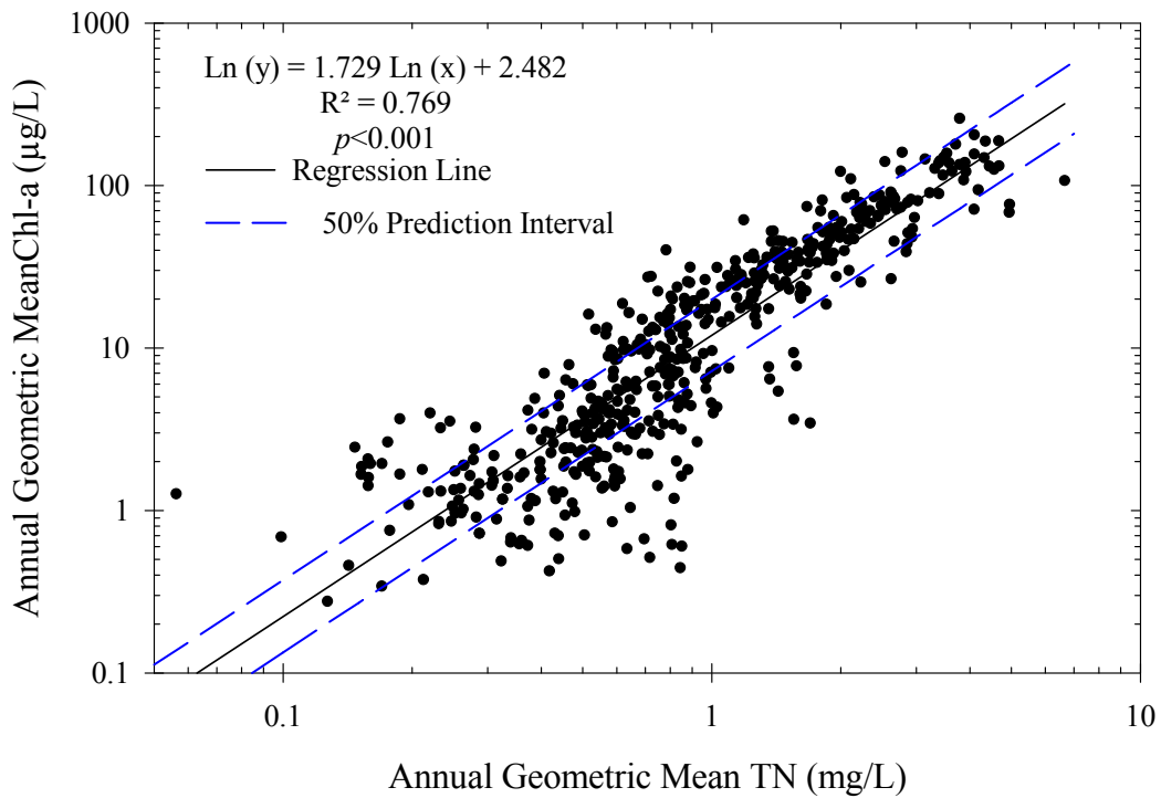
Figure 1-13. Regression analyses annual geometric mean chl. a concentrations and annual geometric mean (A) TP and (B) TN concentrations in clear Florida lakes. Note that x axis and y axis are both expressed on a log-scale.
