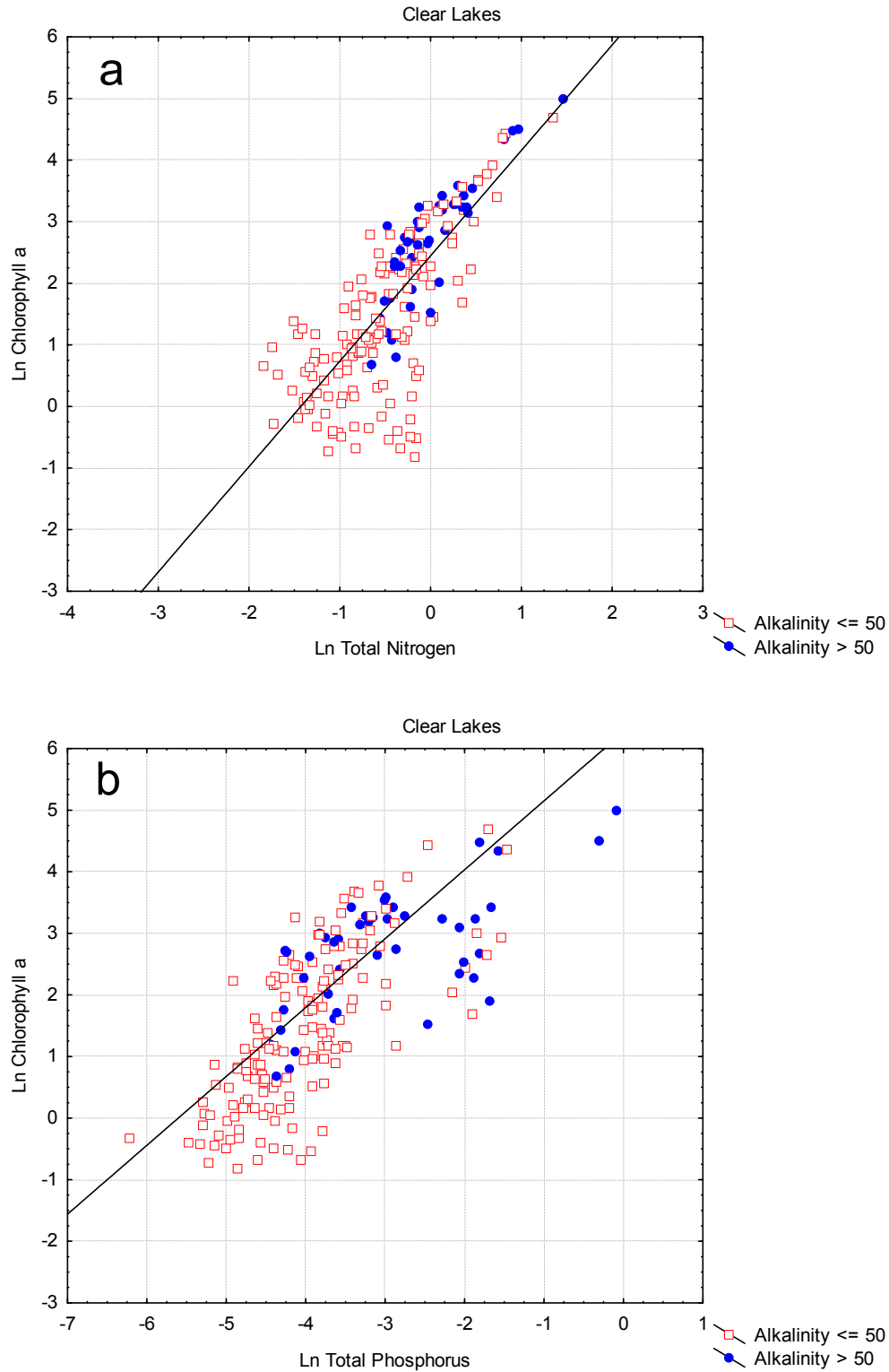
Figure 1-5. Scatter plot of annual geometric mean chl. a concentration and nutrients of clear lakes, showing acidic ( < 50 mg/L \text{CaCO}_3 ) and alkaline lakes. Acidic and alkaline groups were combined in a single regression.
